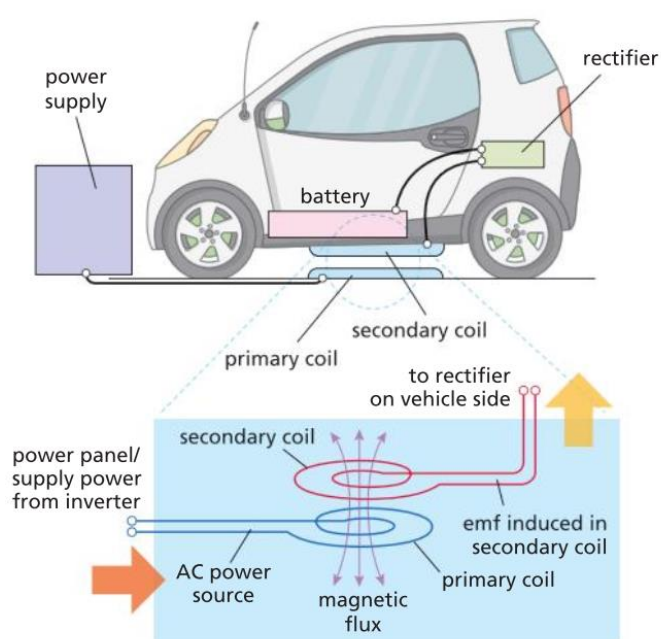
Figure 1 Wireless recharge
